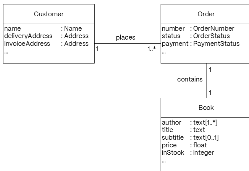
Figure 3.8 Example of a simple UML class diagram
