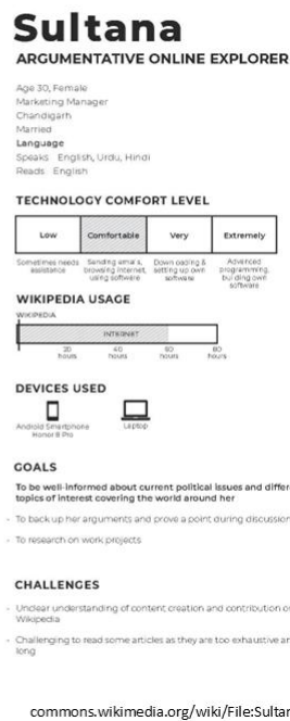
Figure 4.3 Persona example
