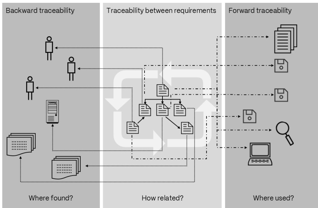
Figure 6.4 Traceability types
